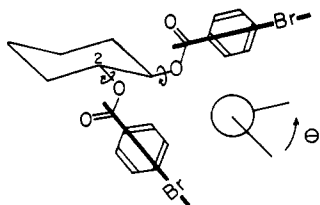
Figure 1. A hypothetical 1(e),2(e)-bis( p -bromobenzoate). The bold lines indicate direction of electric transition moments, which give rise to the UV maximum around 244 nm ( 1 L a band). The chirality of the depicted dibenzoate system is counterclockwise or negative. Curved arrows denote rotational mobility.
