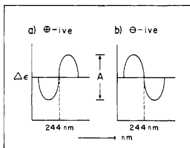
Figure 2. Split Cotton effects centered at 244 nm due to two or more chirally interacting p -bromobenzoates. (a) A positively split CD. (b) A negatively split CD.
