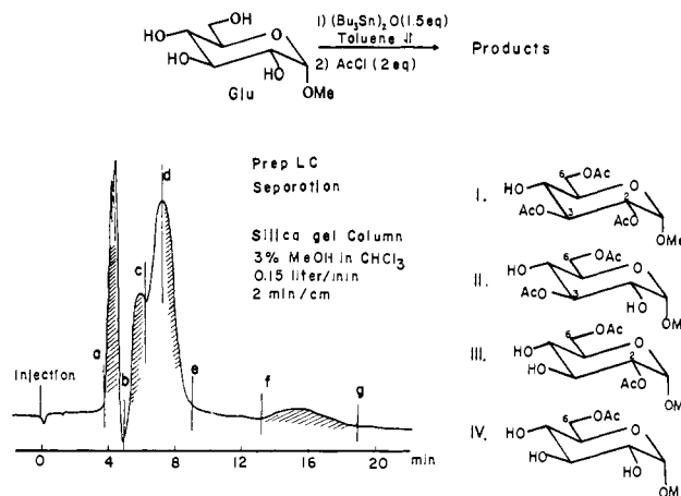
Figure 3. Preparation and prep LC separation of methyl glucoside partial acetates. Shaded fractions a-b, b-c, d-e, and f-g yielded acetates I, II, III, and IV, respectively.
